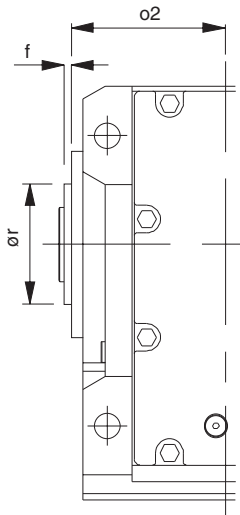
Male spigot K03 - K07
